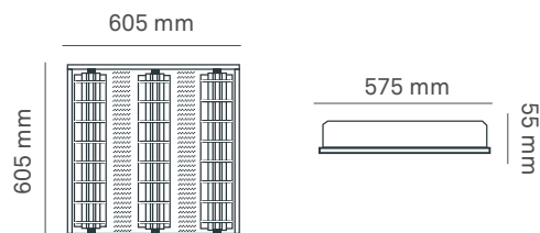
Fluorescente 84 W / LED 54 W
